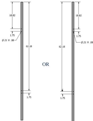
Door Hinged on Right
